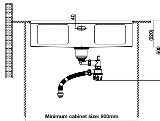
Under-mount
